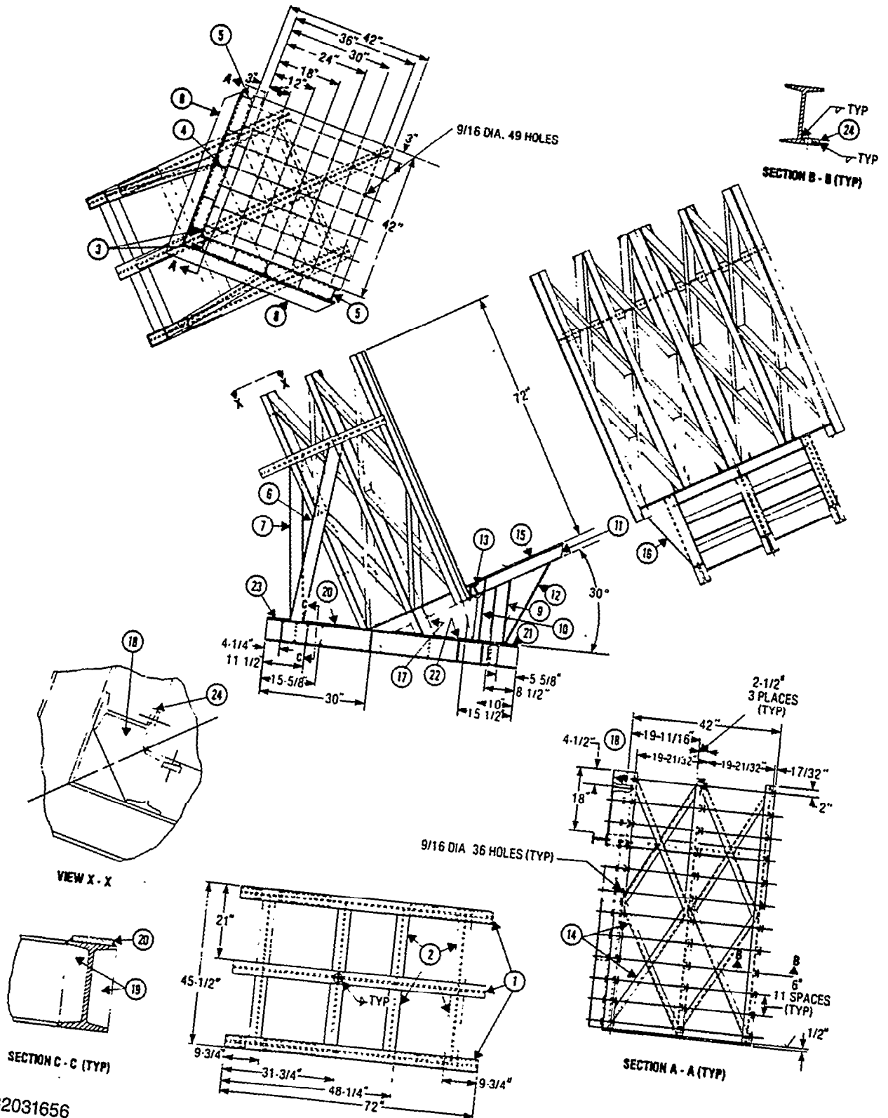
FIGURE 18. 30 degree mounting fixture for testing bulkhead mounted equipment on mediumweight shock testing machine
