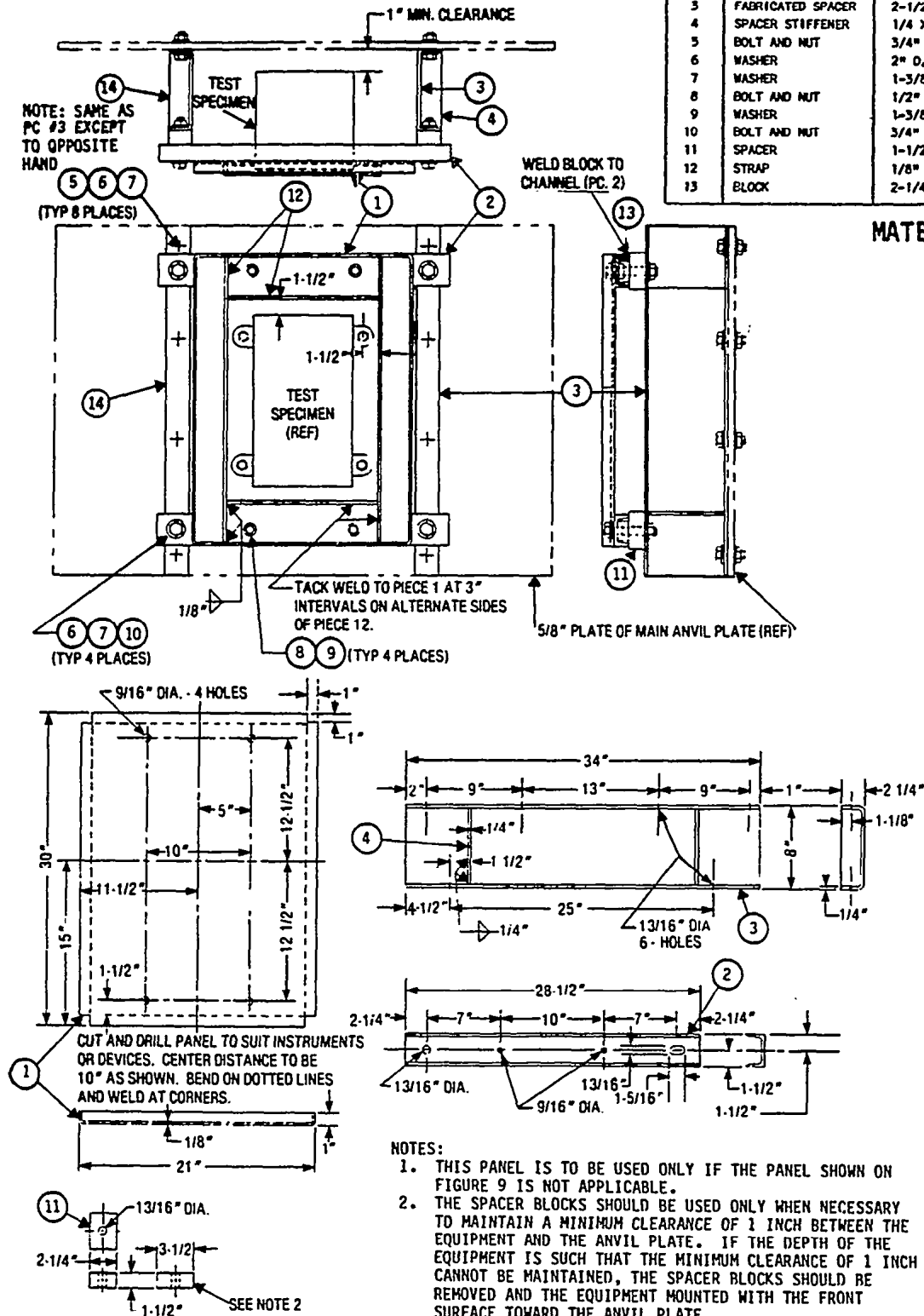
FIGURE 10. Fixture 6D-2 standard mounting for electrical indicating switchboard meters and other panel mounted equipment (type "C" test LWSM).
